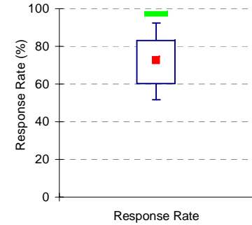
School response rate against Primary School distribution
