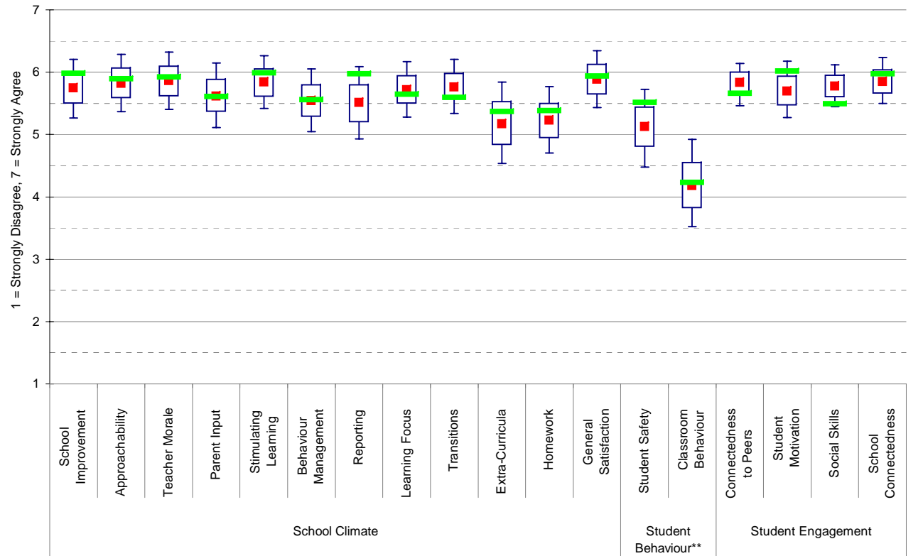
School means plotted against distribution of Primary School means
