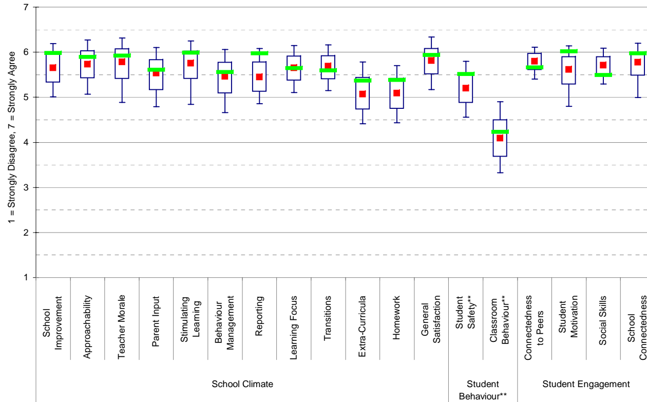
School means plotted against distribution of state-wide school means
