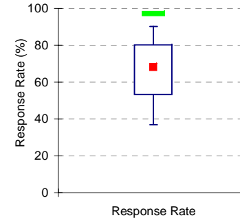
School response rate against state-wide school distribution
